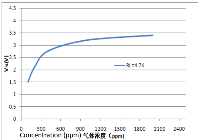
Fig5.Sensivity Curve
